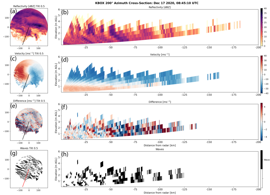
Figure 7. PPIs (a, c, e, g) and RHIs (b, d, f, h) constructed from PPI scans of reflectivity, radial velocity, the difference of radial velocity for successive scans, and the wave detection field for data from the KBOX WSR-88D radar near Boston, MA at 08:45 UTC on 17 December 2020. The RHIs are constructed from data on the 200° azimuth as denoted by the radial line on the PPI panels. An animated version of this figure is in the Video Supplement Animation-Figure-7.
