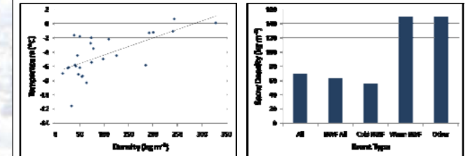
Figure 9. New snowfall density vs. surface temperature at event maturation (left) and new snowfall density by event type (right).
