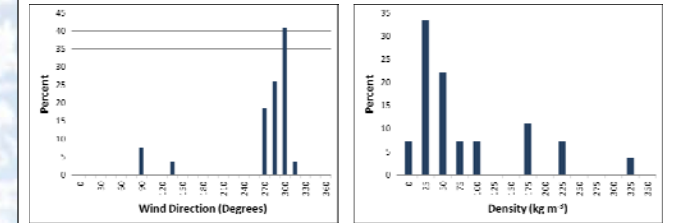
Figure 8. Percent snow events by wind direction (left) and snow density (right).
