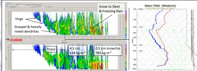
Figure 5a. 16-17 Jan 2008 (4.6 cm, 184 kg m -3 )
