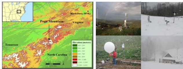
Figure 1. Location of field site and topographic setting (left) and instrumentation (right).
